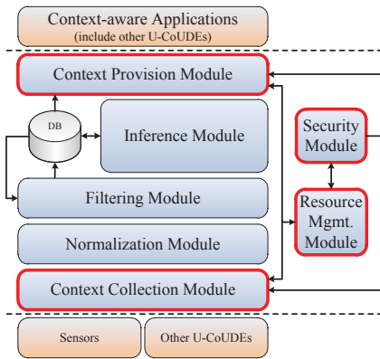
Fig. 1. U-CoUDE architecture.
